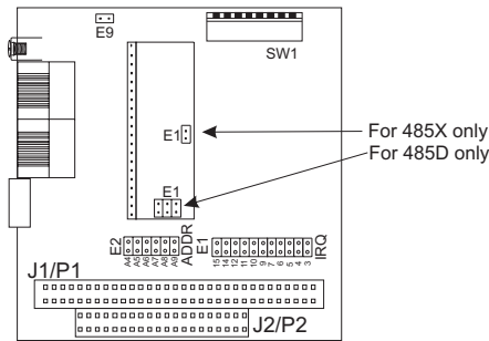
Figure 7—Jumper settings for PC10422 models.
