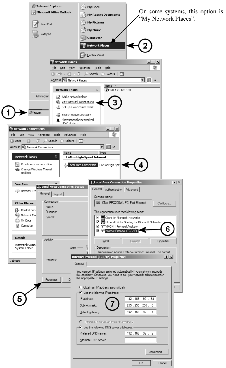
Figure 9 — Steps for Changing the IP Address of the PC Used for Setup
