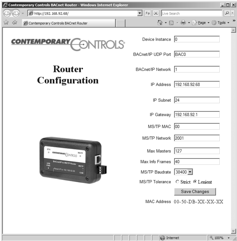
Figure 10 — Router Configuration Page with Default Values
