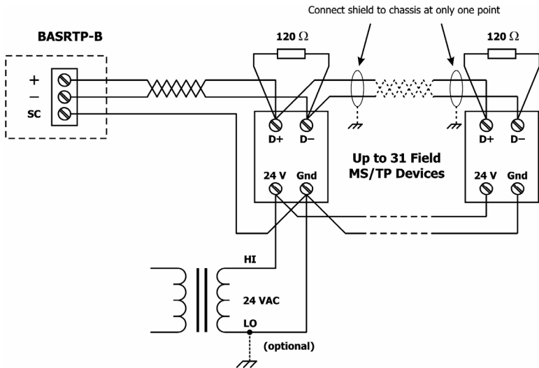
Figure 5 — 2-wire MS/TP Bus Wiring
