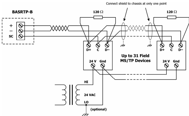
Figure 6 — 3-wire MS/TP Bus Wiring
